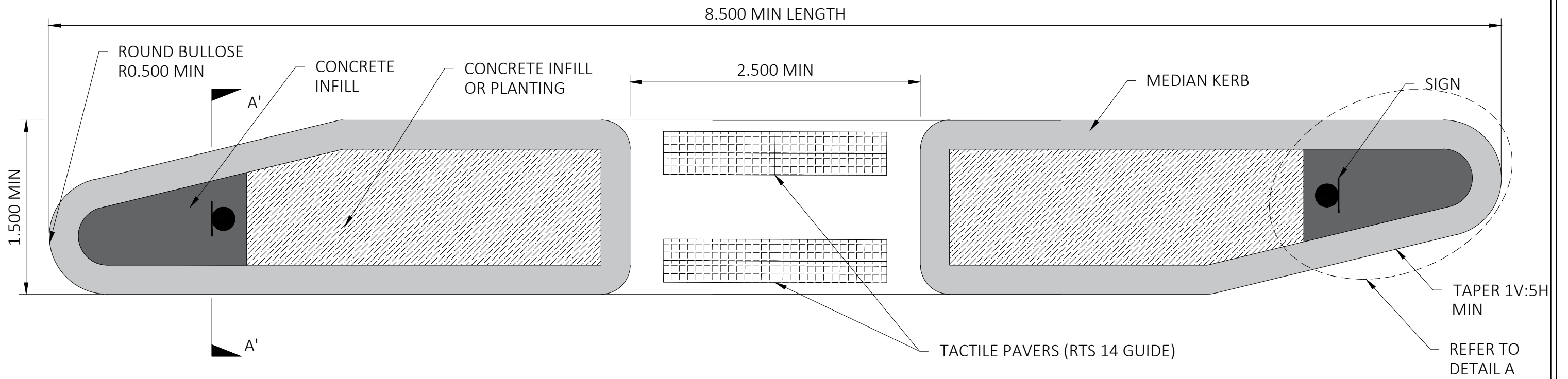
SCHEMATIC PLAN
