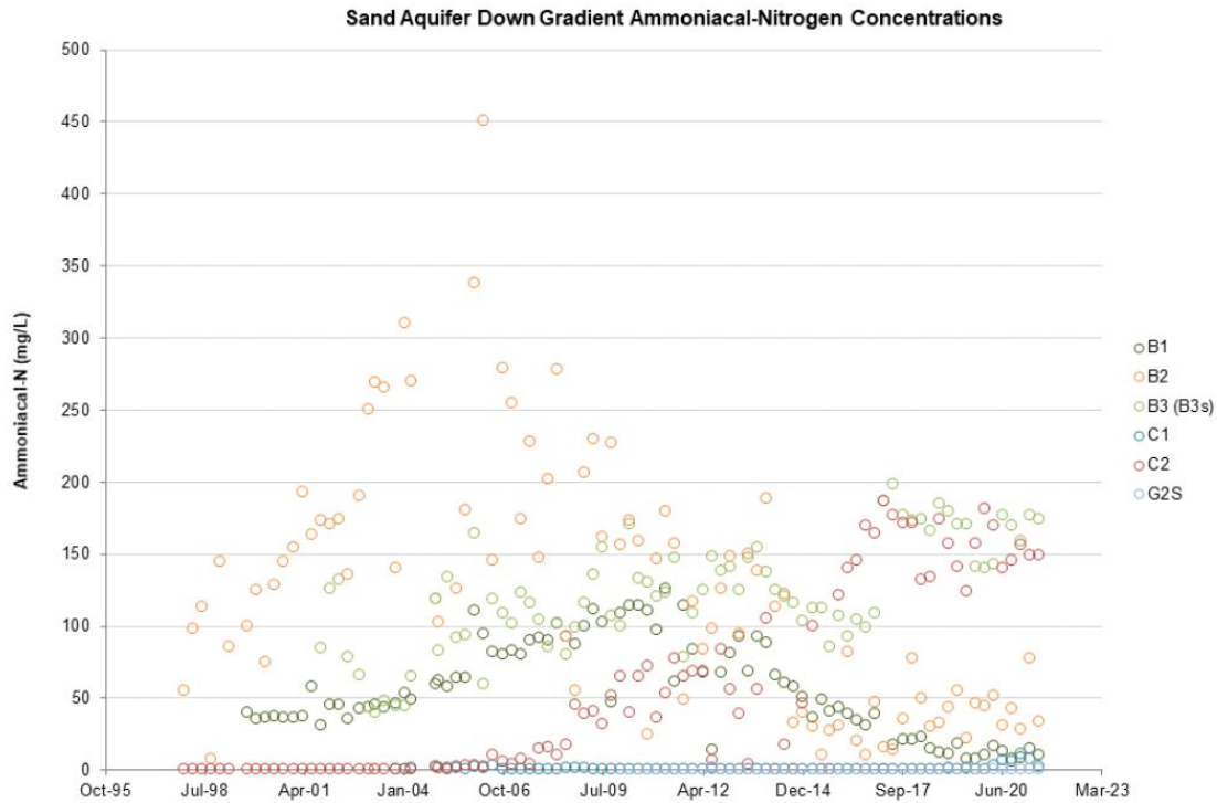
Figure 2: Showings bores samples results for B1, B2, B3 (B3s), C1, C2 and G2S. These are monitoring parameters down gradient of old unlined landfill. For the actual location of bores please see Site Plan in Appendix A of the report.
