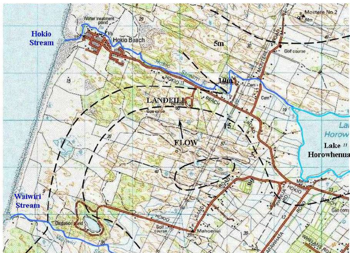
Figure 2-1: Shallow Groundwater Flow Direction
